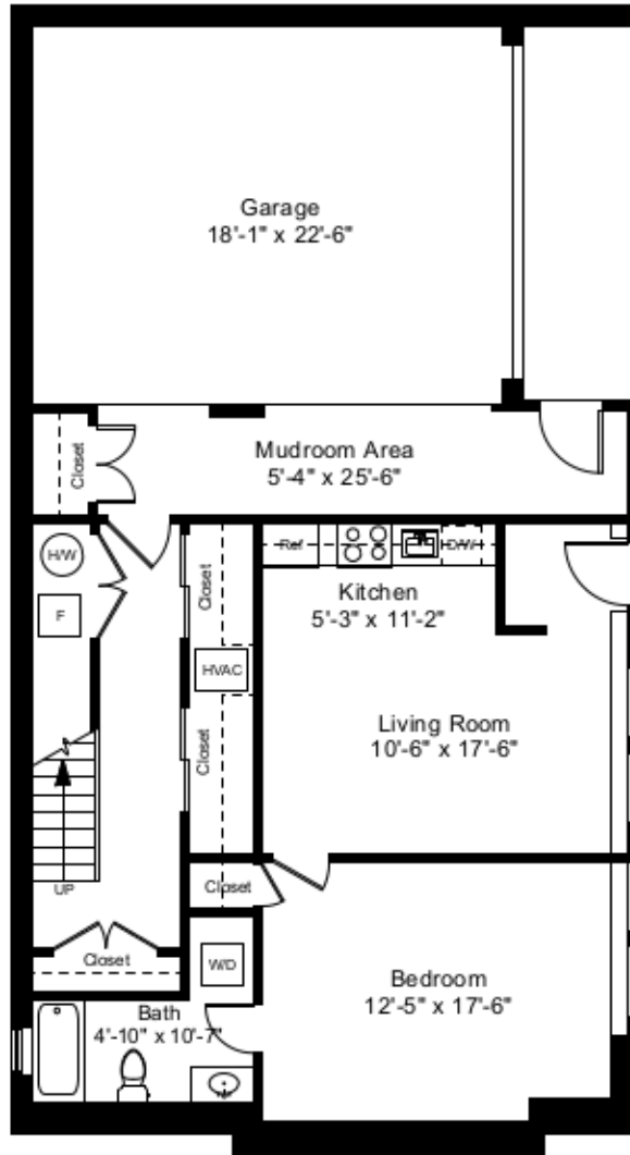
Lower Level Plan Ceiling Height = 7'-5"
